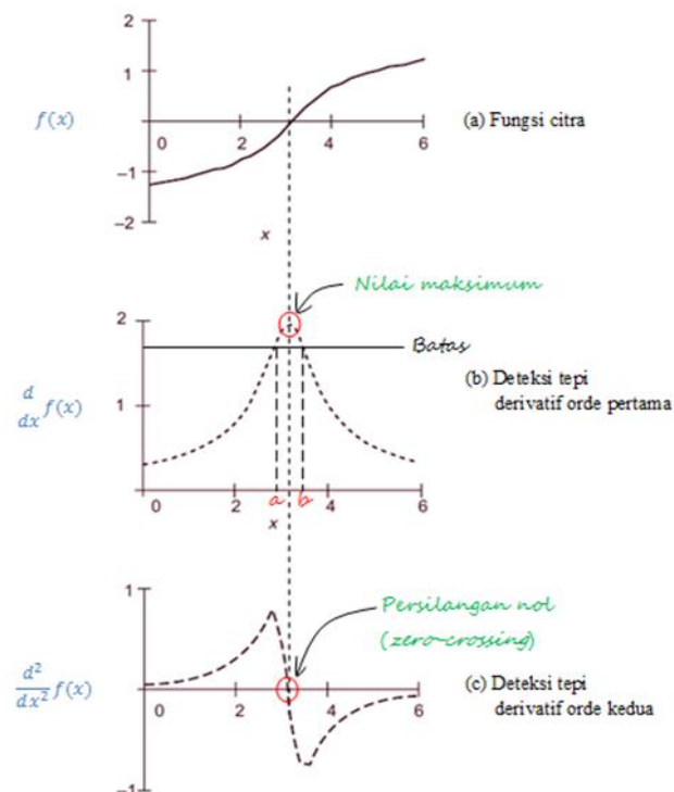
Figure 1. First and Second edge Detection in X area
