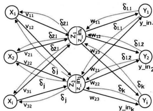
Figure 2. ANN Backpropagation Treatment Process
