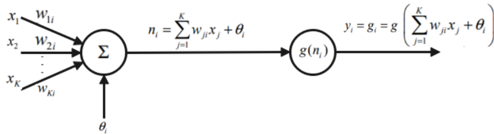
Figure 2. FFNN network
