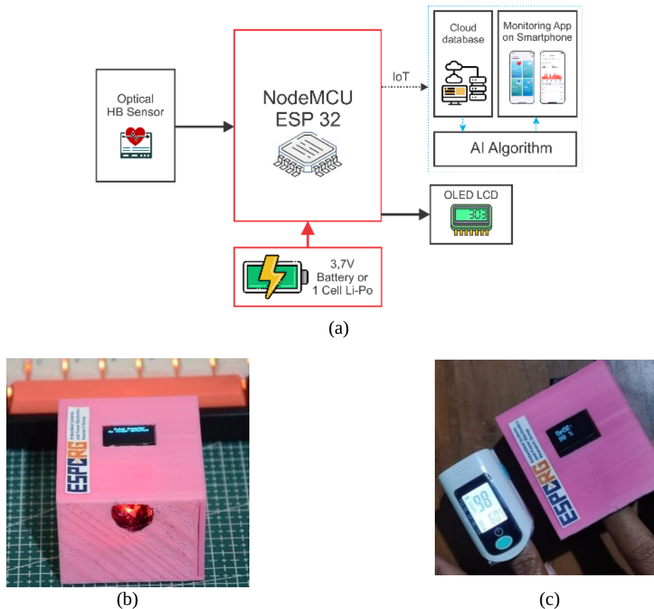
Figure 2. Experimental device developed by author: (a) diagram block of the system, (b) device front view, and (c) developed device calibration process.
