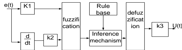
Figure 7. Basic Structure of Fuzzy Logic Controller
