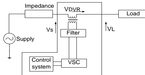
Figure 1. Basic Structure of Dynamic Voltage Restorer.
