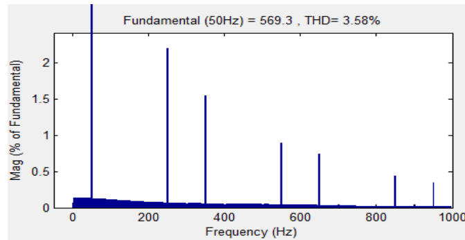
Figure 12. THD for Voltage with Fuzzy Controller
