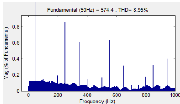
Figure 11. THD for Voltage with PI Controller
