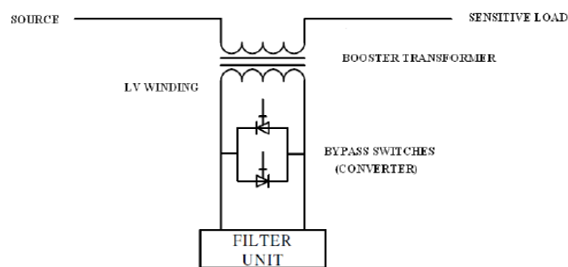
Figure 3. Standby Mode of DVR
