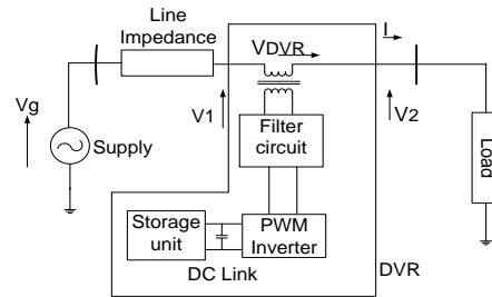
Figure 5. Block Diagram of General DVR Circuit
