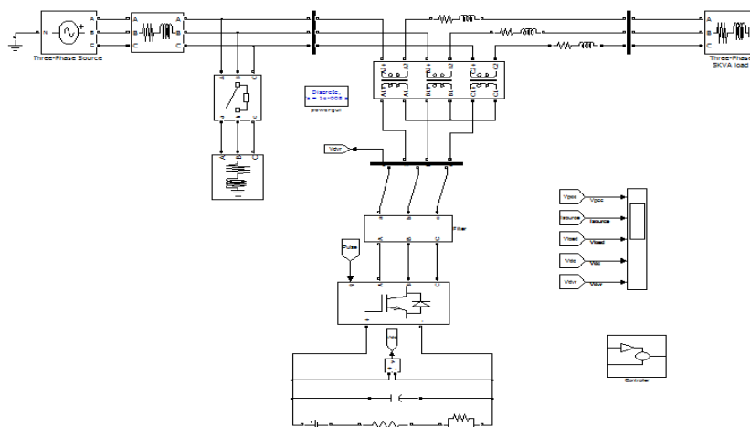
Figure 8. Simulation Diagram for Dynamic Voltage Restorer
