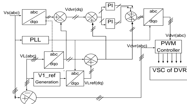
Figure 6. Control Block Diagram for DVR
