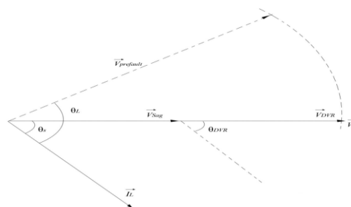
Figure 4. In-Phase Compensation Method
